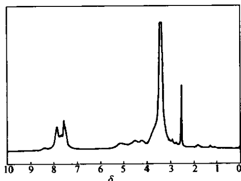
Fig. 2 ^1\text{H-NMR} spectrum of PHCS3
