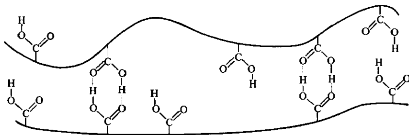
Fig. 5 Schematic representation of structure for amic acid-chitosan molecules in solution, showing that the occurrence of random interchain di-association of macromolecular carboxylic acid avoids liquid crystal ordering
