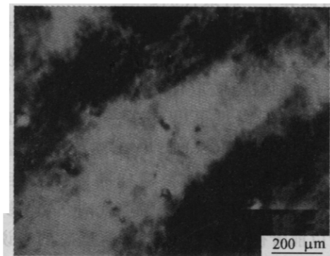
Fig. 4 Polarized optical micrograph of 20 wt% PHCS6/DCA solution, showing a typical liquid crystalline texture
